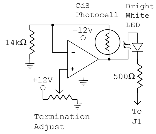
Termination Control Circuit - Use Single-Supply Op Amp
