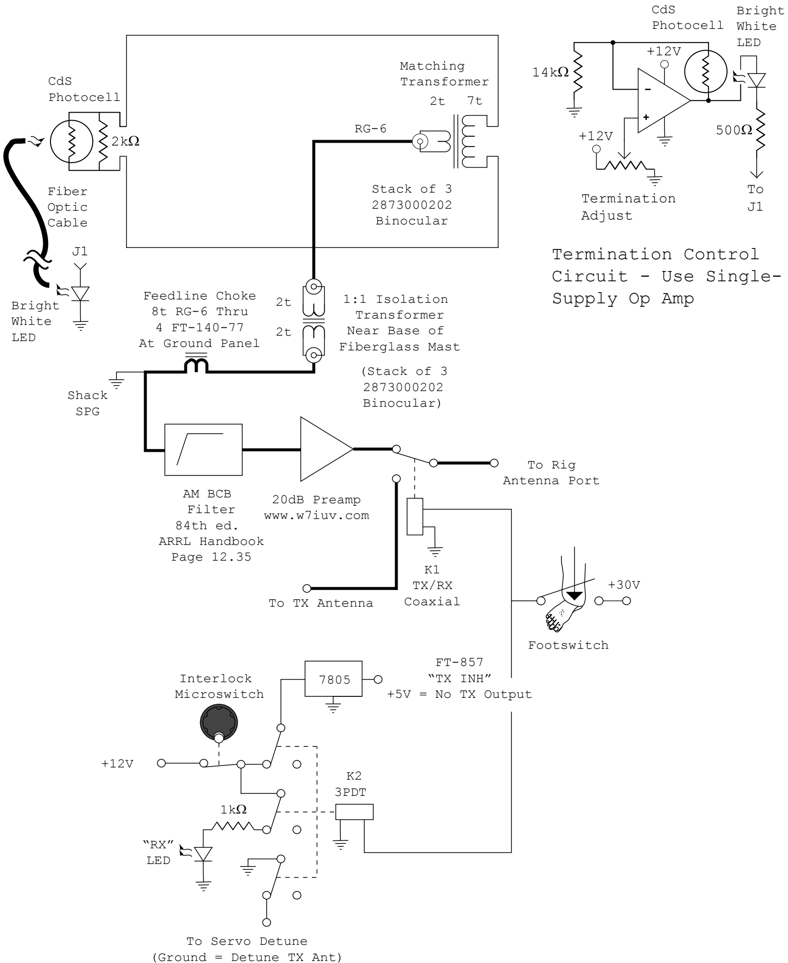
Flag System Schematic - N3OX
